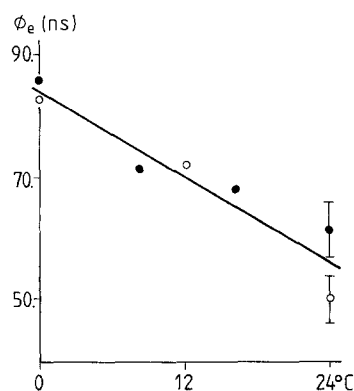
Fig. 4. Equivalent rotational correlation time (339 nm) of the single tryptophan residue in the bacteriophage M13 coat protein incorporated in DOPC (—○—) and mixed DOPC/DOPG bilayers (80/20 w/w) (—●—) as a function of temperature (°C) after excitation at 300 nm. The L/P ratio is 35 and 41, respectively
