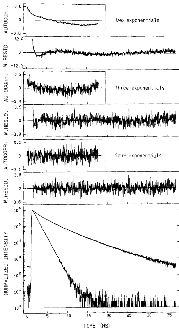
Fig. 1. Fluorescence decay at 339 nm of the single tryptophan residue in bacteriophage M13 coat protein incorporated in DMPC/DMPG (80/20, w/w) after excitation at 300 nm at 0°C. Also shown is the fluorescence response of p -terphenyl in ethanol. The L/P ratio is 8. The fit channel range is from 40 to 1024 (36 ps/channel). The parameters describing the fit with 4 exponentials are \alpha_1 = 0.18 \pm 0.01 , \alpha_2 = 0.33 \pm 0.02 , \alpha_3 = 0.46 \pm 0.02 , \alpha_4 = 0.04 \pm 0.01 , \tau_1 = 0.37 \pm 0.05 ns, \tau_2 = 1.89 \pm 0.11 ns, \tau_3 = 4.65 \pm 0.16 ns, \tau_4 = 10.25 \pm 0.72 ns. The upper panels represent the residuals and the autocorrelation function of the residuals for the fit with 2, 3 and 4 exponentials, respectively. The \chi^2 values for these fits are 2.30, 1.12 and 0.99, respectively. The Durbin-Watson parameters are 0.68, 1.76 and 1.97, respectively. The numbers of zero passages in the autocorrelation function are 14, 188 and 246, respectively.
