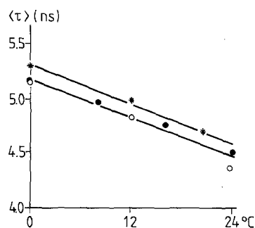
Fig. 2. Average fluorescence lifetime at 339 nm as a function of temperature (°C) of the single tryptophan residue of bacteriophage M13 coat protein incorporated in DOPC (—○—), DOPC/DOPG (80/20 w/w) (—●—) and mixed DMPC/DMPG (80/20 w/w) (—*—) with L/P = 35, 41, 38, respectively, after excitation at 300 nm.
