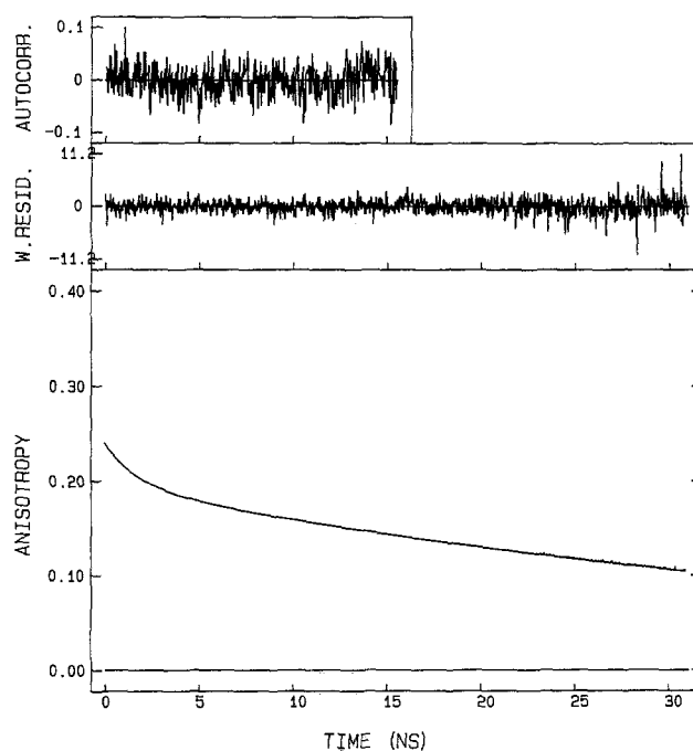
Fig. 3. Fluorescence anisotropy decay (339 nm) at 24°C of the single tryptophan residue in bacteriophage M13 coat protein incorporated in DOPC bilayers with L/P = 35 after excitation at 300 nm. The fit from channels 40 to 1024 (33 ps/channel) is a dual exponential function with \beta_1 = 0.056 \pm 0.003 , \beta_2 = 0.196 \pm 0.003 , \phi_1 = 1.6 \pm 0.2 ns and \phi_2 = 50 \pm 4 ns. The \chi^2 value and the Durbin-Watson parameter are 0.98 and 1.96, respectively. The number of zero passages of the parallel intensity component is 230, of the perpendicular intensity component is 264.
